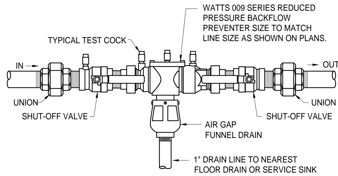
BACKFLOW PREVENTER DETAIL NO SCALE
