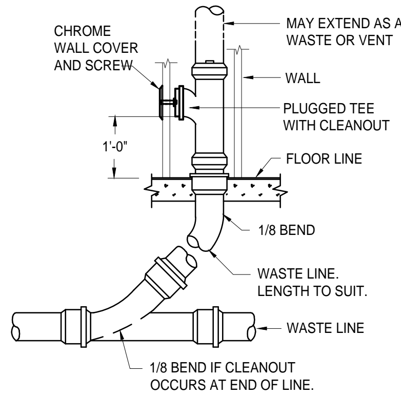
WALL CLEANOUT DETAIL NO SCALE
